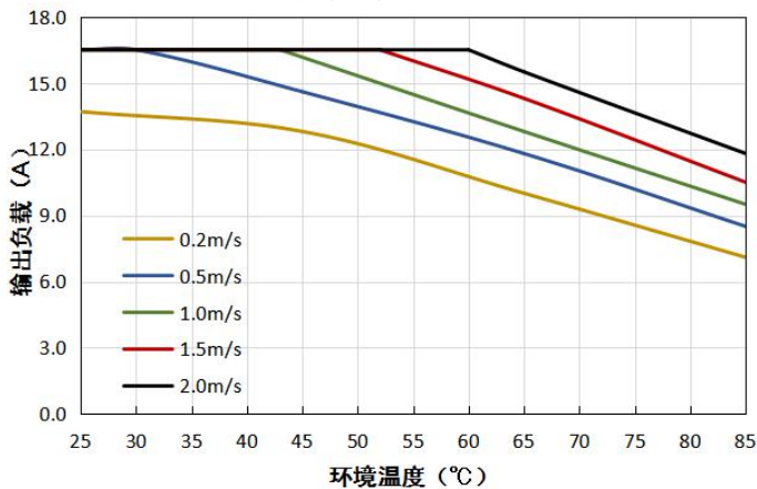
VCF4824QBO-400WHR3(-N) 温度降额曲线 (Vin=48V)
