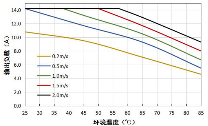
VCF4828QBO-400WHR3(-N) 温度降额曲线 (Vin=48V)
