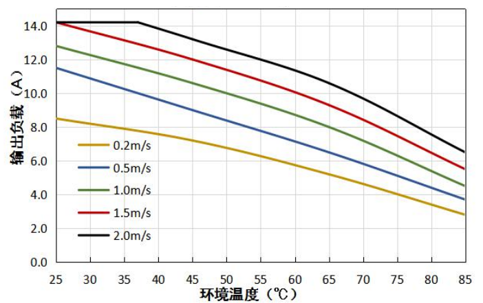
VCF4828QBO-400WR3(-N) 温度降额曲线 (Vin=48V)
