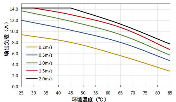
VCF4828QBO-400WFR3(-N) 温度降额曲线 (Vin=48V)
